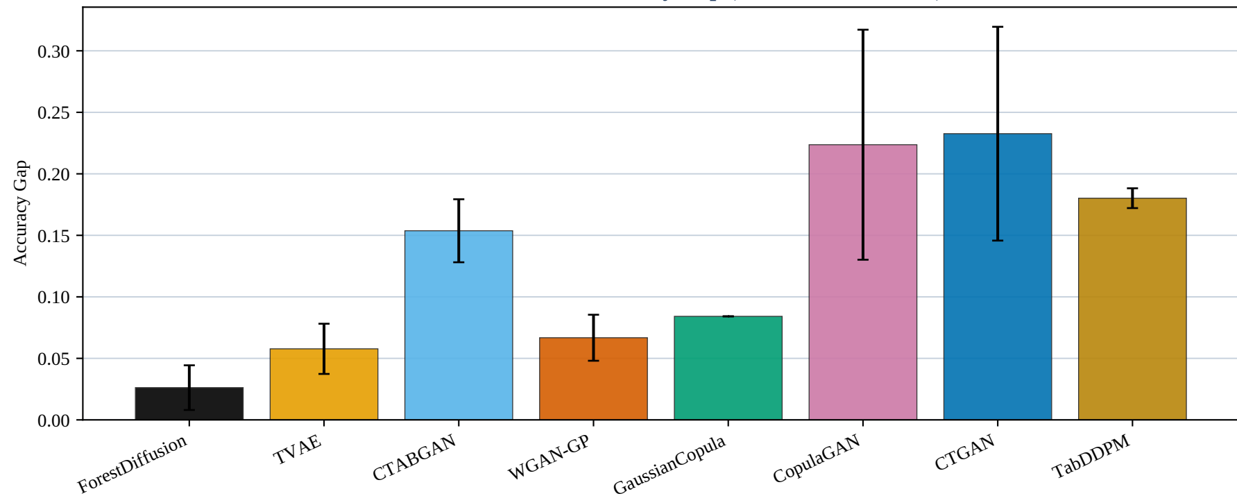
MAGIC Gamma — Accuracy Gap (mean \pm SD, 10 seeds)
